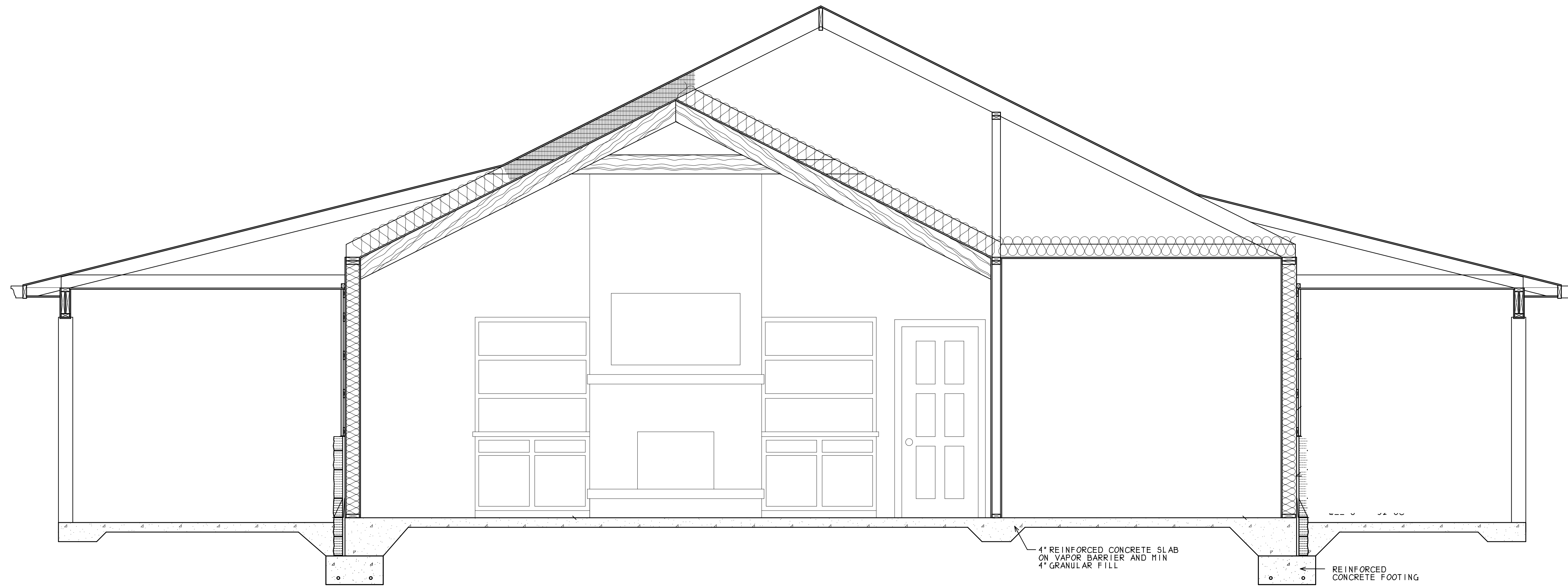
CROSS SECTION
