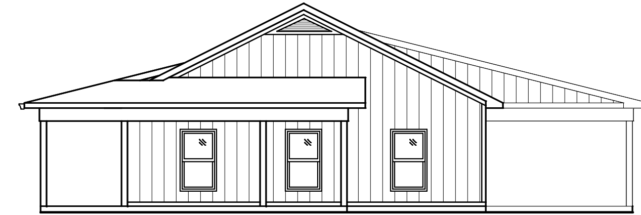
WEST ELEVATION
