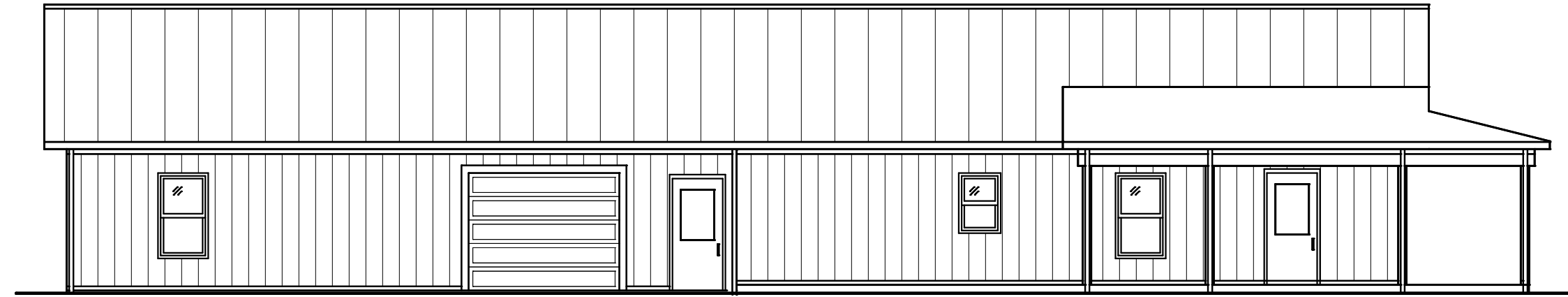
FRONT ELEVATION
