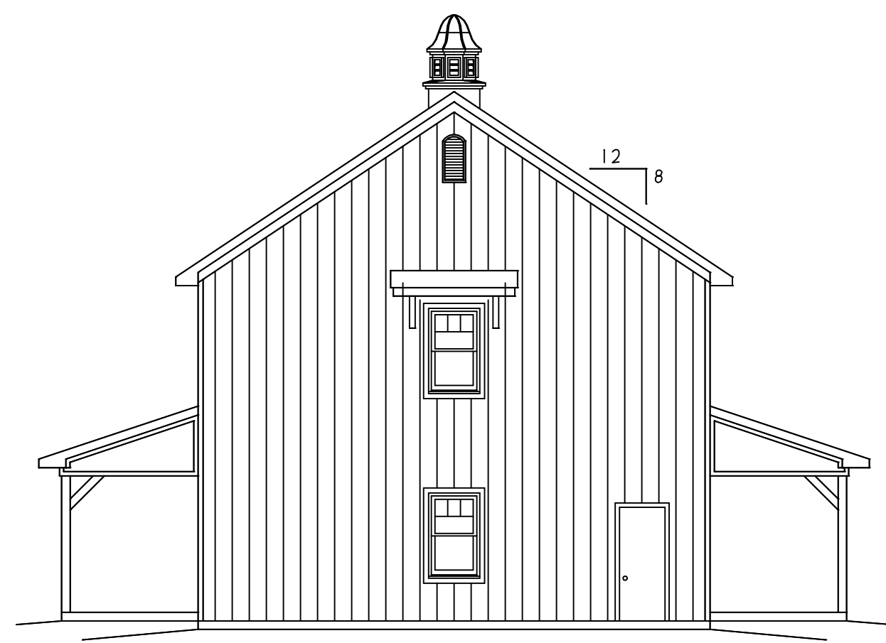
WEST ELEVATION
