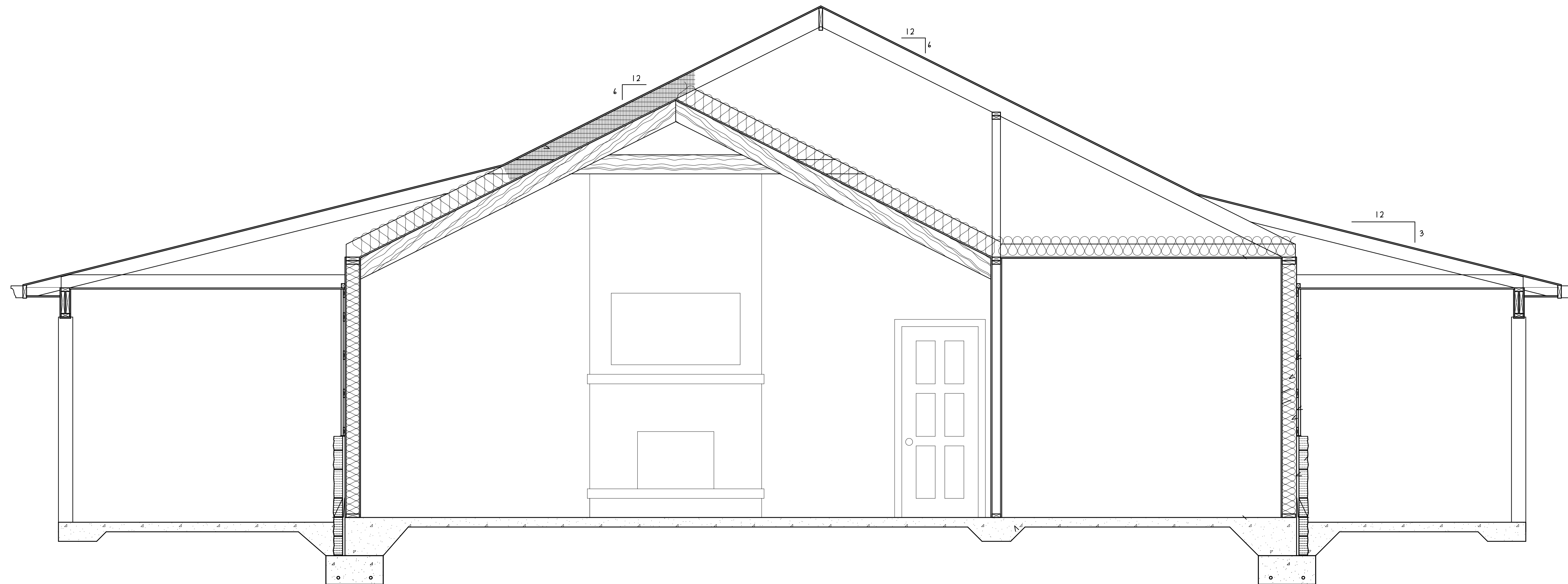
CROSS SECTION
